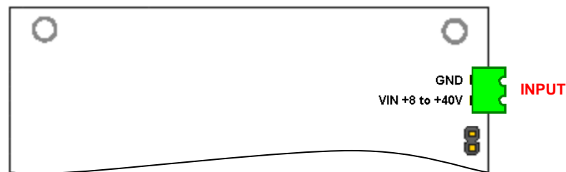
Figure 7. Input power connector
