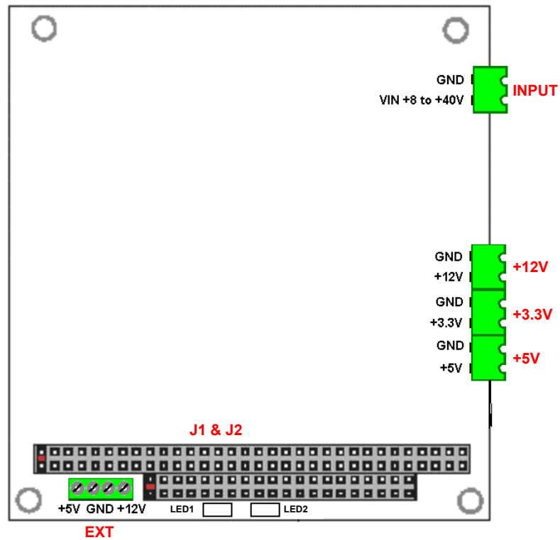
Figure 4. Connector layout
