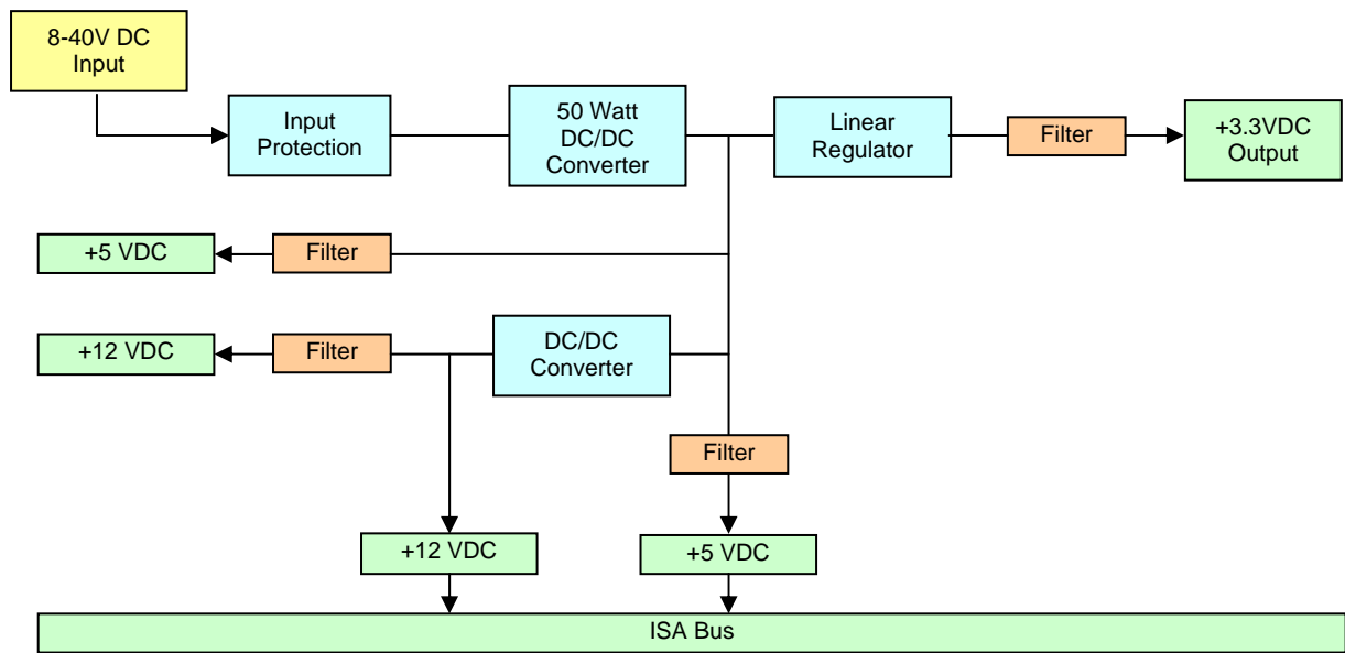
Figure 2. Functional block diagram of the ACS-5151 vehicle class power supply
