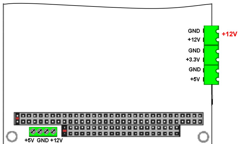
Figure 8. +12V output connector
